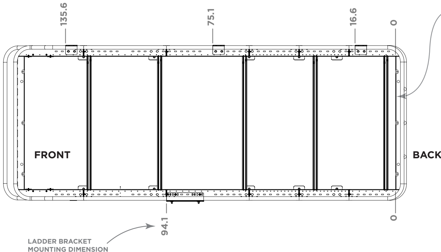
REFERENCE POINT
