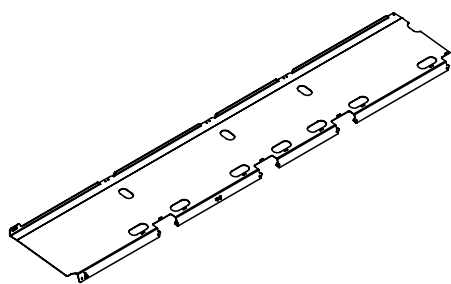
170 DRIVER FRONT CEILING PANEL
